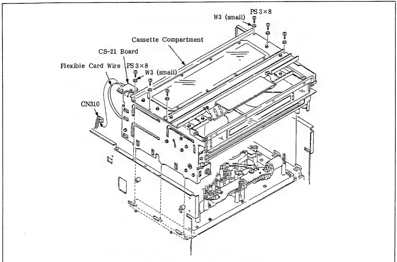
Fig. 6-11 Replacement of the Cassette Compartment
